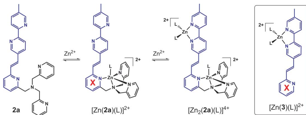
Fig. 9 Three coordination states of 2a along a \text{Zn}^{2+} gradient. L: coordinating solvent. Note that \text{Zn}^{2+} resides at different ends of the fluorophore in the monozinc complexes of 2a and 3 . The red crosses highlight the difference in coordination status of this pyridyl group in the monozinc complexes of ditopic 2a and monotopic 3 .
